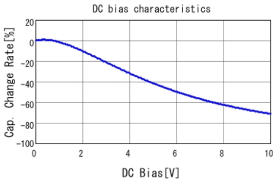
■ GRM32EB31A476KE20 C-DC bias capchange, 20.0degC, AC0.
