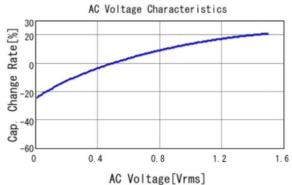
■ GRM32EB31A476KE20 C-AC Voltage capchange, DCOV, 20.0d
