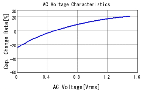
■ GRM32EB31A476ME20 C-AC Voltage capchange, DCOV, 20.0d
