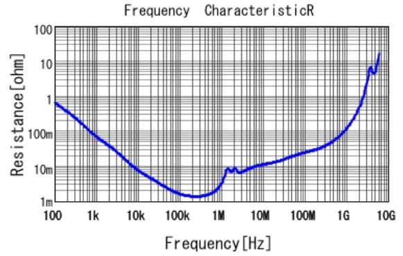
■ GRM32EB31C476ME15 R DCOV, 20degC
