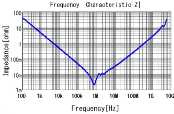
■ GRM32EB31C476ME15 |Z| DCOV, 20degC
