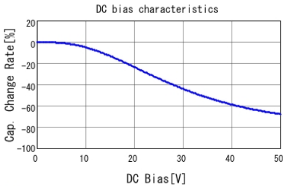
■ GRM32EB31H475KA87 C-DC bias capchange, 20.0degC, AC1.
