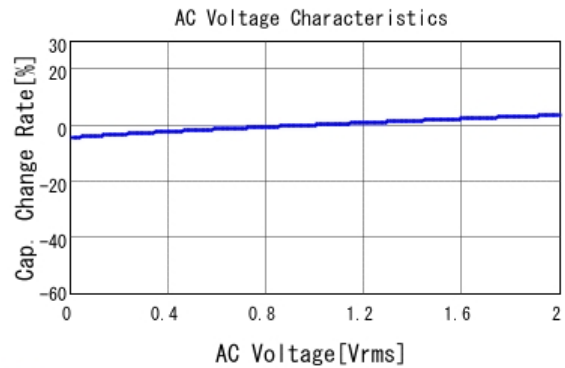
■ GRM32EB31H475KA87 C-AC Voltage capchange, DCOV, 20.0d
