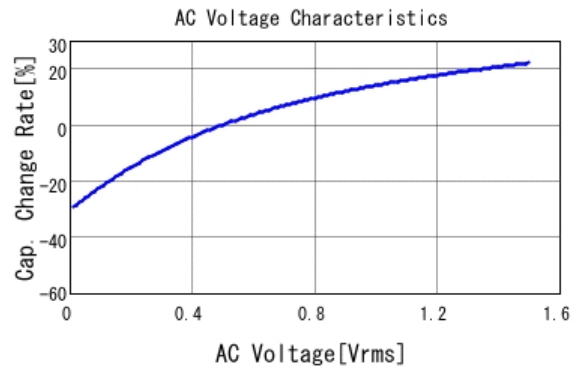
■ GRM32EC81E226KE15 C-AC Voltage capchange, DCOV, 25.0d
