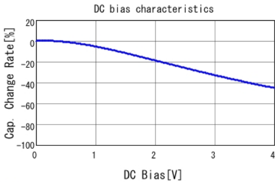
■ GRM32EE70G107ME19 C-DC bias capchange, 25.0degC, AC0.
