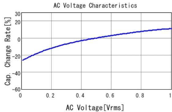
■ GRM32EE70G107ME19 C-AC Voltage capchange, DCOV, 25.0d
