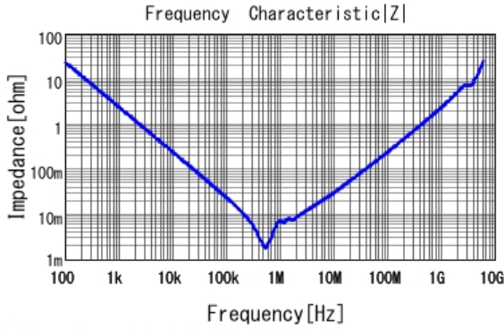
■ GRM32EE70G107ME19 |Z| DCOV, 25degC
