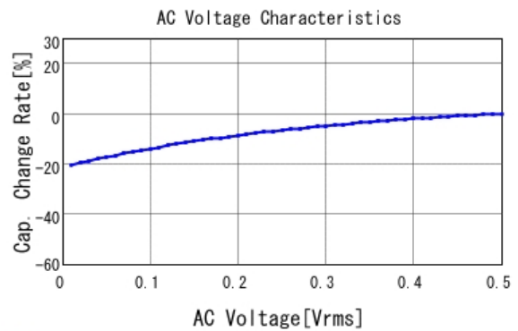
■ GRM32ER60G337ME05 C-AC Voltage capchange, DCOV, 25.0d
