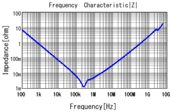
■ GRM32ER60G337ME05 |Z| DCOV, 25degC
