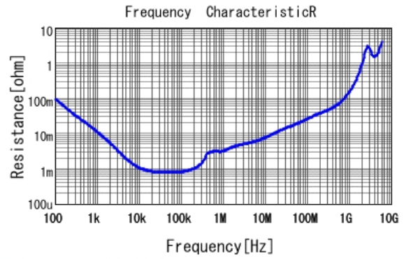
■ GRM32ER60G337ME05 R DCOV, 25degC
