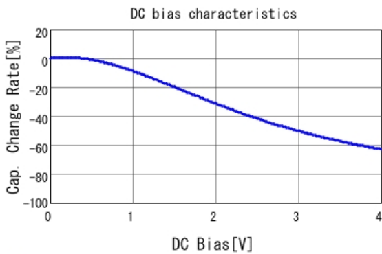
■ GRM32ER60G337ME05 C-DC bias capchange, 25.0degC, AC0.
