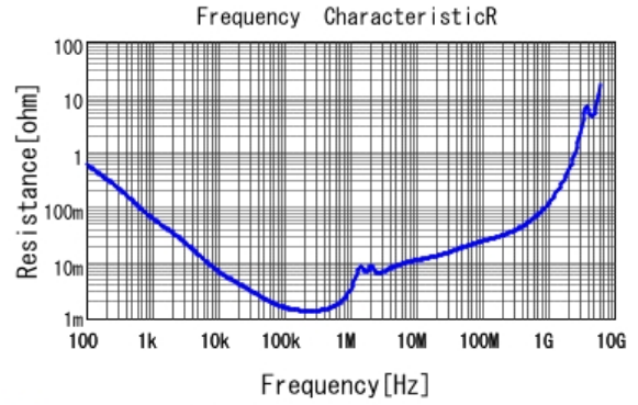
■ GRM32ER60J476ME20 R DCOV, 25degC
