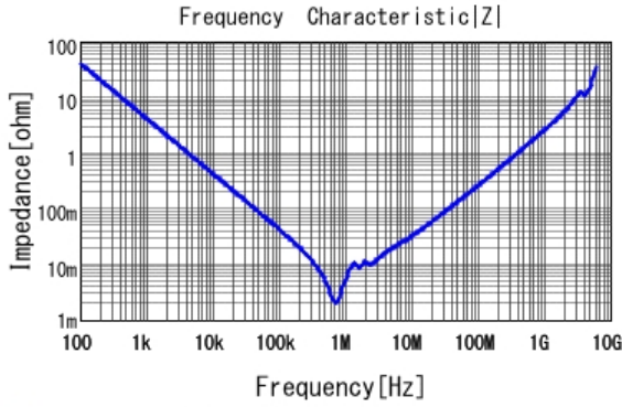
■ GRM32ER60J476ME20 |Z| DCOV, 25degC
