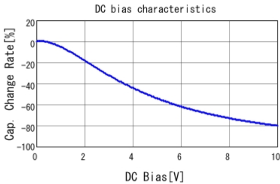
■ GRM32ER61A107ME20 C-DC bias capchange, 25.0degC, AC0.
