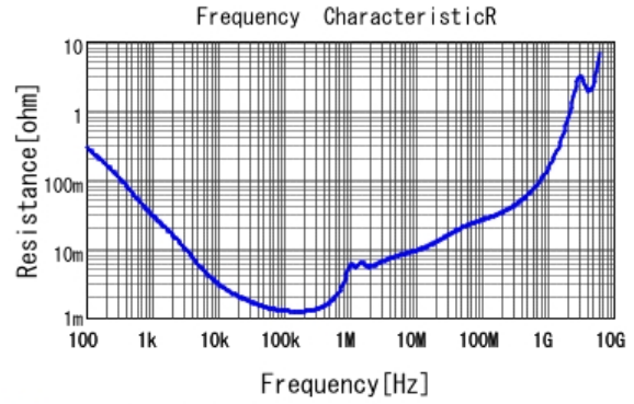
■ GRM32ER61A107ME20 R DCOV, 25degC
