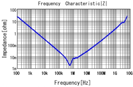
■ GRM32ER61A107ME20 |Z| DCOV, 25degC
