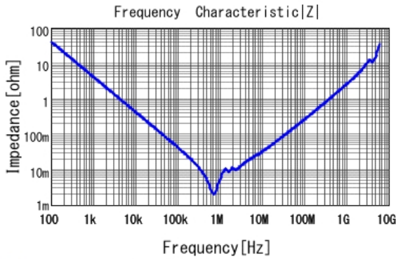
■ GRM32ER61A476KE20 |Z| DCOV, 25degC
