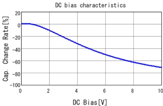
■ GRM32ER61A476KE20 C-DC bias capchange, 25.0degC, AC0.
