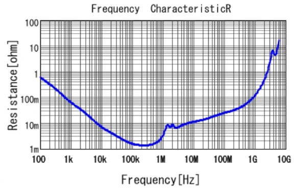
■ GRM32ER61A476KE20 R DCOV, 25degC
