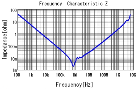
■ GRM32ER61C476ME15 |Z| DCOV, 25degC
