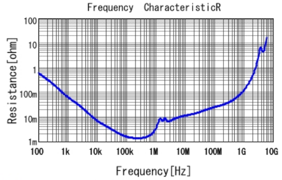
■ GRM32ER61C476ME15 R DCOV, 25degC
