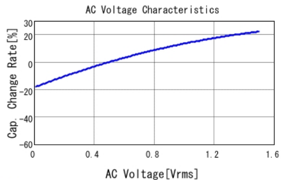
■ GRM32ER61E226KE15 C-AC Voltage capchange, DCOV, 25.0d
