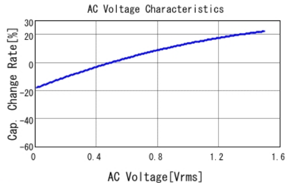
■ GRM32ER61E226ME15 C-AC Voltage capchange, DCOV, 25.0d
