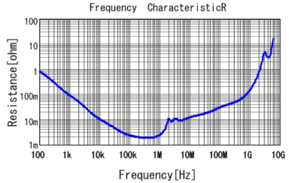
■ GRM32ER61E226ME15 R DCOV, 25degC
