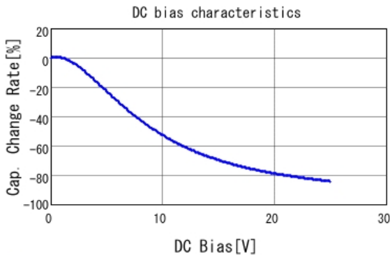
■ GRM32ER61E226ME15 C-DC bias capchange, 25.0degC, AC0.
