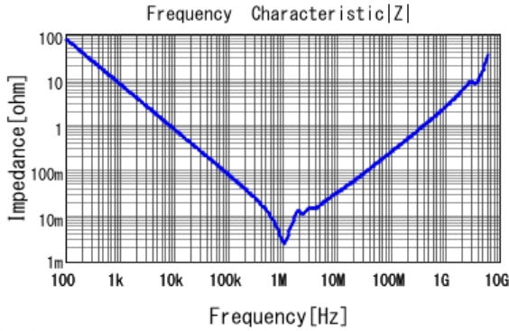
■ GRM32ER61E226ME15 |Z| DCOV, 25degC
