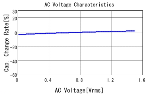
■ GRM32ER61H106KA12 C-AC Voltage capchange, DCOV, 25.0d
