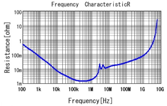
■ GRM32ER61H106KA12 R DCOV, 25degC
