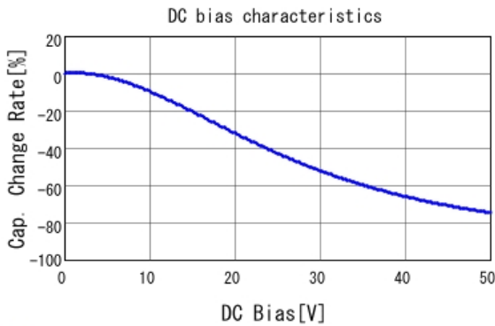
■ GRM32ER61H106KA12 C-DC bias capchange, 25.0degC, AC1.
