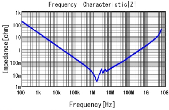
■ GRM32ER61H106KA12 |Z| DCOV, 25degC
