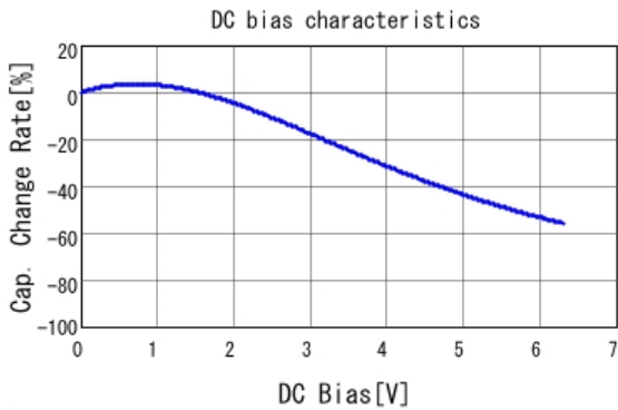
■ GRM32ER70J476ME20 C-DC bias capchange, 25.0degC, AC0.
