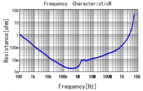
■ GRM32ER70J476ME20 R DCOV, 25degC
