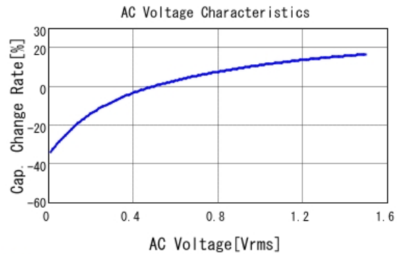
■ GRM32ER70J476ME20 C-AC Voltage capchange, DCOV, 25.0d
