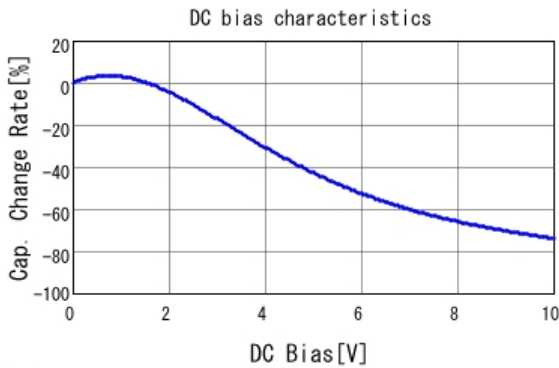
■ GRM32ER71A476KE15 C-DC bias capchange, 25.0degC, AC0.
