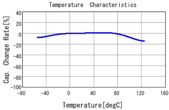
■ GRM32ER71A476KE15 C-Temp. capchange, DC0.0V, AC0.5Vrm
