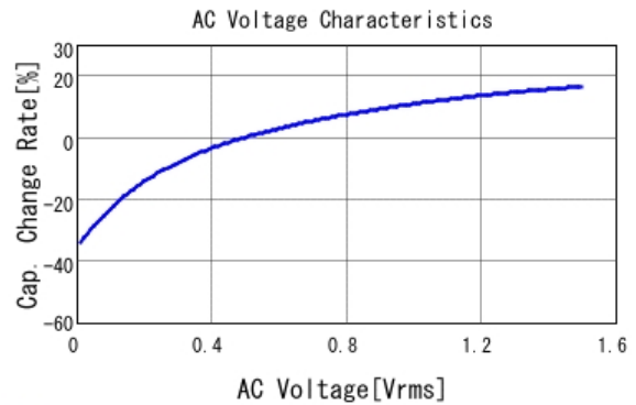
■ GRM32ER71A476KE15 C-AC Voltage capchange, DCOV, 25.0d
