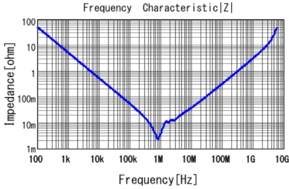
■ GRM32ER71A476KE15 |Z| DCOV, 25degC
