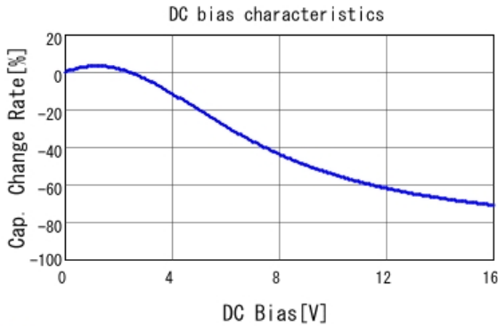
■ GRM32ER71C226MEA8 C-DC bias capchange, 25.0degC, AC0.
