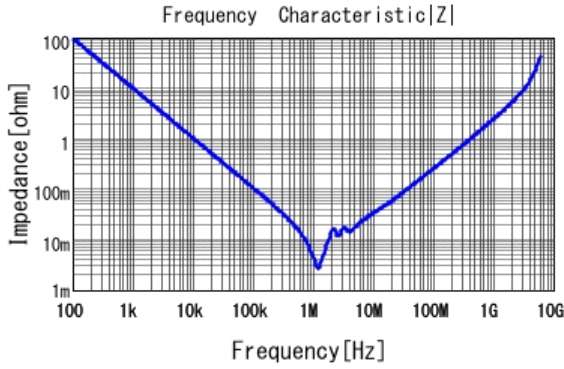
■ GRM32ER71C226MEA8 |Z| DCOV, 25degC
