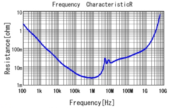
■ GRM32ER71H475KA88 R DCOV, 25degC
