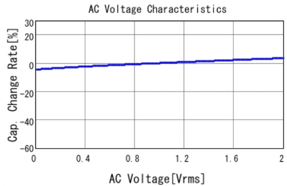
■ GRM32ER71H475KA88 C-AC Voltage capchange, DCOV, 25.0d
