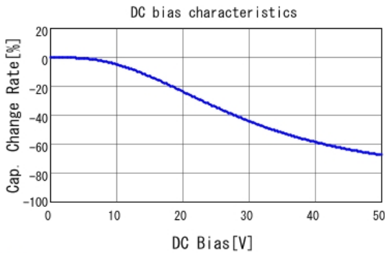
■ GRM32ER71H475KA88 C-DC bias capchange, 25.0degC, AC1.
