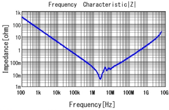
■ GRM32ER71H475KA88 |Z| DCOV, 25degC
