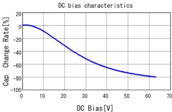
■ GRM32ER71J106KA12 C-DC bias capchange, 25.0degC, AC1V
