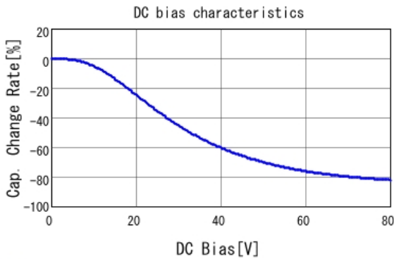
■ GRM32ER71K475KE14 C-DC bias capchange, 25.0degC, AC1.
