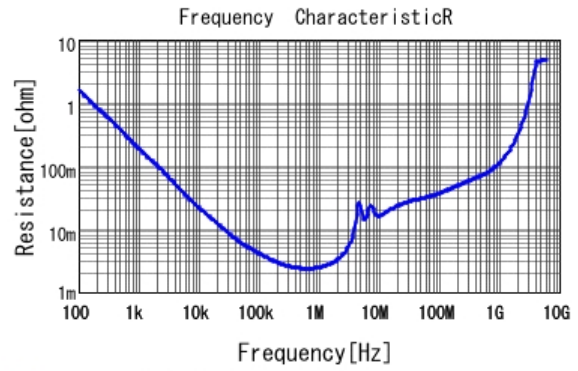
■ GRM32ER71K475KE14 R DCOV, 25degC
