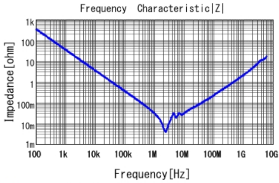
■ GRM32ER71K475KE14 |Z| DCOV, 25degC
