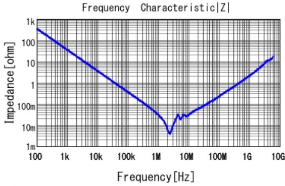
■ GRM32ER71K475ME14 |Z| DCOV, 25degC
