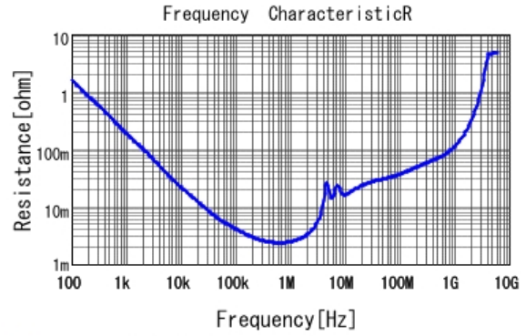
■ GRM32ER71K475ME14 R DCOV, 25degC
