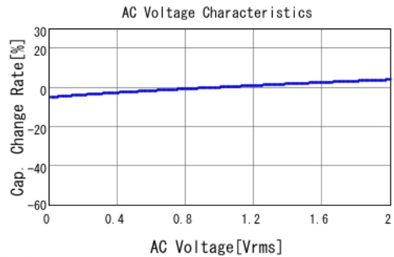
■ GRM32ER71K475ME14 C-AC Voltage capchange, DCOV, 25.0d
