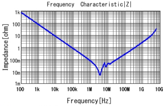
■ GRM32ER72A225KA35 |Z| DCOV, 25degC
