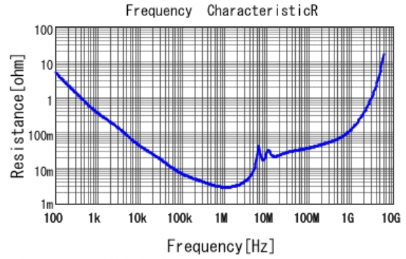
■ GRM32ER72A225KA35 R DCOV, 25degC
