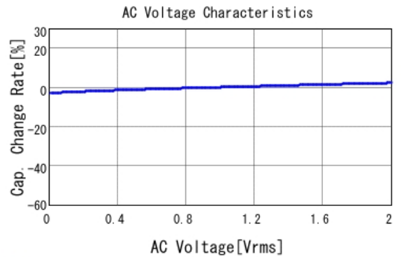
■ GRM32ER72A225KA35 C-AC Voltage capchange, DCOV, 25.0d
