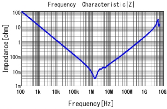
■ GRM32NC81C226ME15 |Z| DCOV, 25degC
