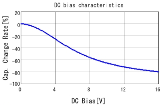
■ GRM32NC81C226ME15 C-DC bias capchange, 25.0degC, AC0.
