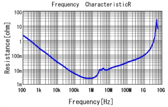
■ GRM32NC81C226ME15 R DCOV, 25degC
