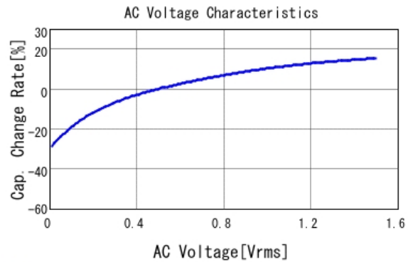
■ GRM32NC81C226ME15 C-AC Voltage capchange, DCOV, 25.0d
