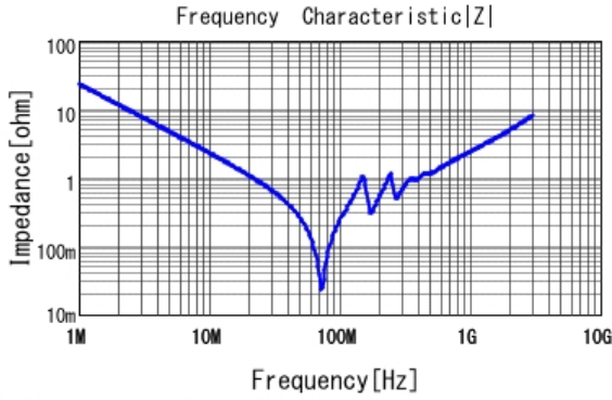
■ GRM32Q7U2J682JW31 |Z| DCOV, 25degC
