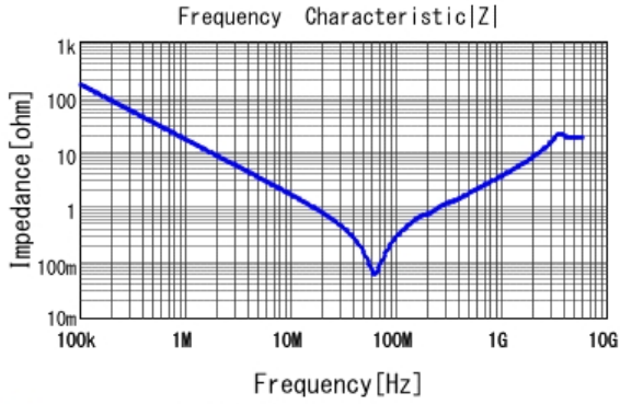
■ GRM32QR73A103KW01 |Z| DCOV, 25degC
