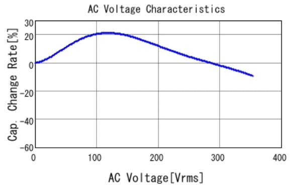
■ GRM32QR73A103KW01 C-AC Voltage capchange, DCOV, 25.0d
