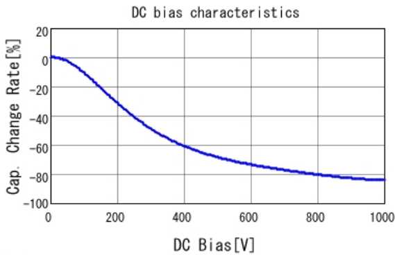
■ GRM32QR73A103KW01 C-DC bias capchange, 25.0degC, AC1V
