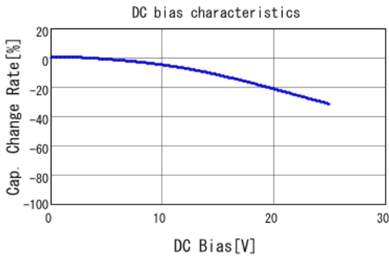
■ GRM32RR71E225KA01 C-DC bias capchange, 25.0degC, AC1.
