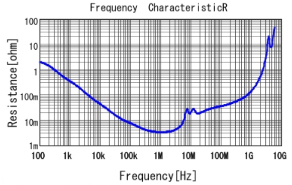
■ GRM32RR71E225KA01 R DCOV, 25degC
