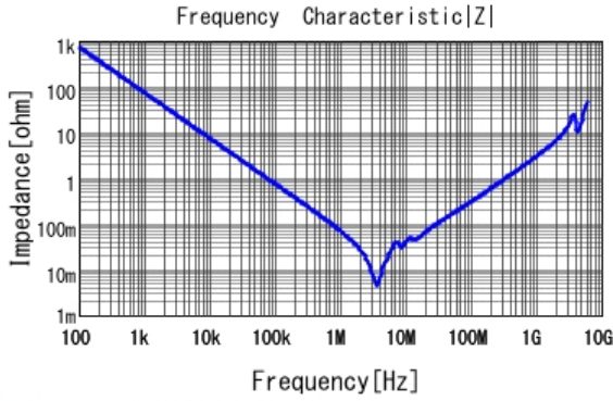
■ GRM32RR71E225KA01 |Z| DCOV, 25degC
