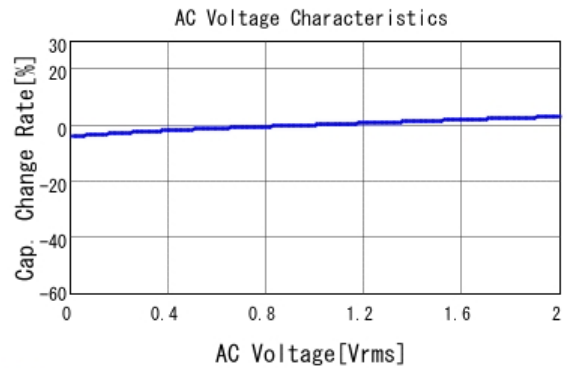
■ GRM32RR71E225KA01 C-AC Voltage capchange, DCOV, 25.0d
