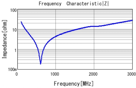
■ GRM42A7U3F680JW31 |Z| DC0V, 25degC
