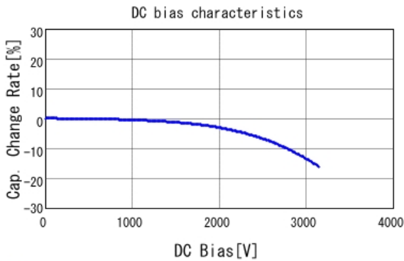
■ GRM42A7U3F680JW31 C-DC bias capchange, 25.0degC, AC1V
