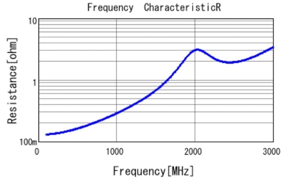
■ GRM42A7U3F680JW31 R DC0V, 25degC
