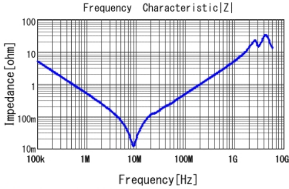
■ GRM43DR72E334KW01 |Z| DCOV, 25degC
