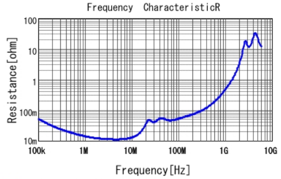
■ GRM43DR72E334KW01 R DCOV, 25degC
