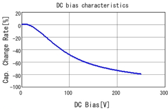
■ GRM43DR72E334KW01 C-DC bias capchange, 25.0degC, AC1V
