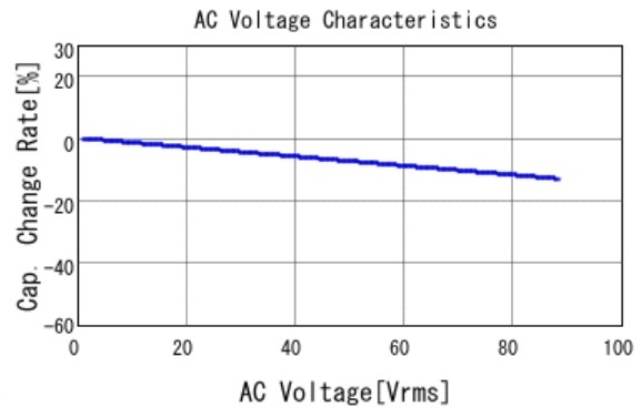
■ GRM43DR72E334KW01 C-AC Voltage capchange, DCOV, 25.0d
