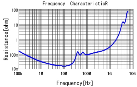
■ GRM43DR72J104KW01 R DCOV, 25degC
