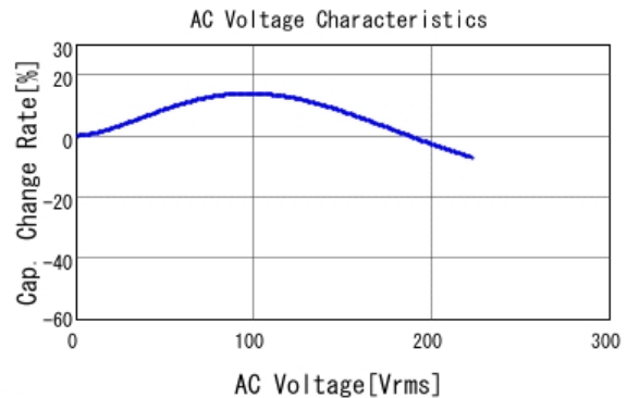
■ GRM43DR72J104KW01 C-AC Voltage capchange, DCOV, 25.0d
