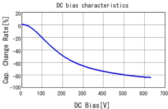
■ GRM43DR72J104KW01 C-DC bias capchange, 25.0degC, AC1V
