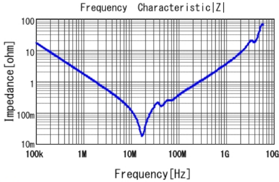
■ GRM43DR72J104KW01 |Z| DCOV, 25degC
