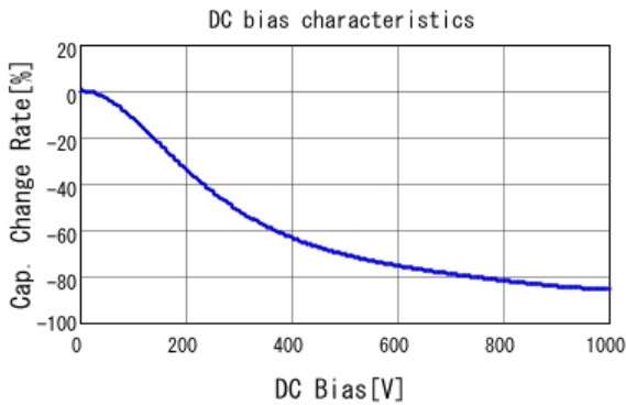
■ GRM43DR73A333KW01 C-DC bias capchange, 25.0degC, AC1V
