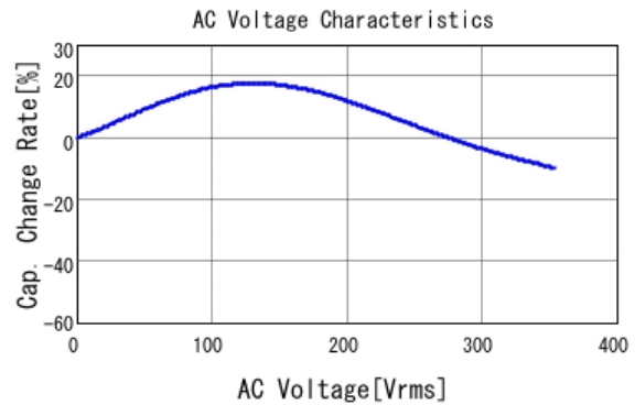
■ GRM43DR73A333KW01 C-AC Voltage capchange, DCOV, 25.0d
