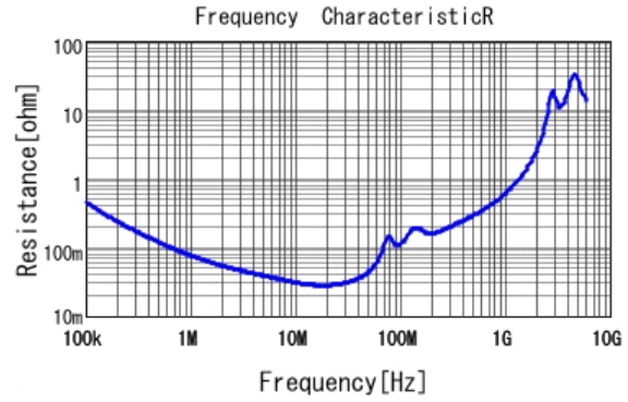
■ GRM43DR73A333KW01 R DCOV, 25degC
