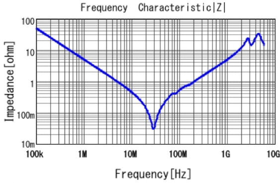
■ GRM43DR73A333KW01 |Z| DCOV, 25degC
