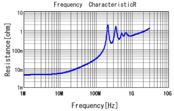
■ GRM43Q7U3A332JW31 R DCOV, 25degC
