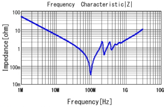
■ GRM43Q7U3A332JW31 |Z| DCOV, 25degC
