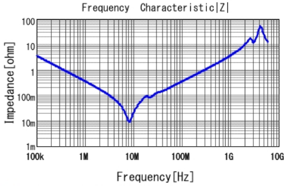
■ GRM55DR72E474KW01 |Z| DC0V, 25degC
