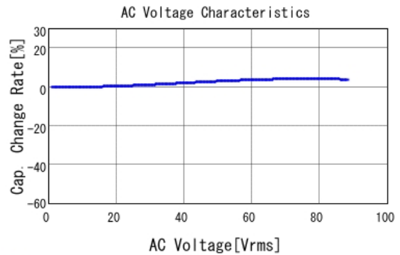
■ GRM55DR72E474KW01 C-AC Voltage capchange, DC0V, 25.0d
