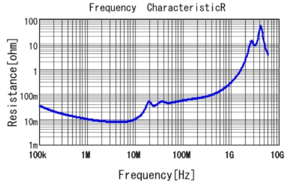
■ GRM55DR72E474KW01 R DC0V, 25degC
