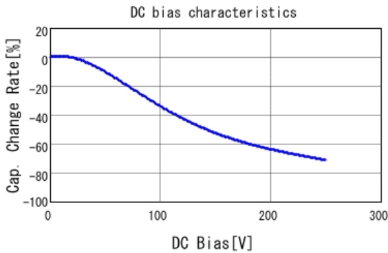
■ GRM55DR72E474KW01 C-DC bias capchange, 25.0degC, AC1V
