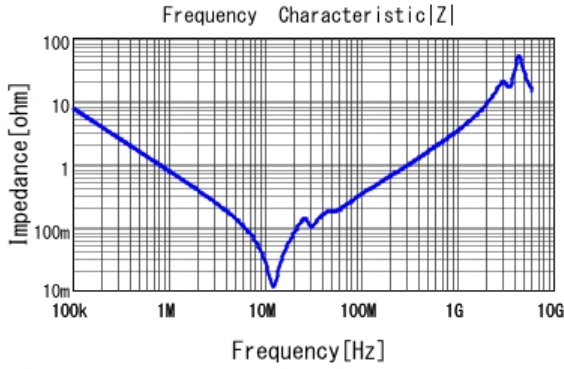
■ GRM55DR72J224KW01 |Z| DC0V, 25degC
