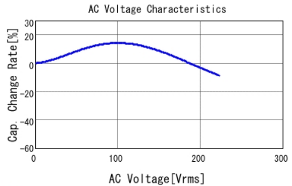
■ GRM55DR72J224KW01 C-AC Voltage capchange, DC0V, 25.0d
