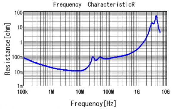
■ GRM55DR72J224KW01 R DC0V, 25degC
