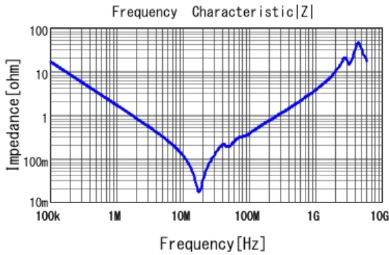
■ GRM55DR73A104KW01 |Z| DC0V, 25degC
