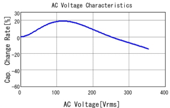
■ GRM55DR73A104KW01 C-AC Voltage capchange, DC0V, 25.0d
