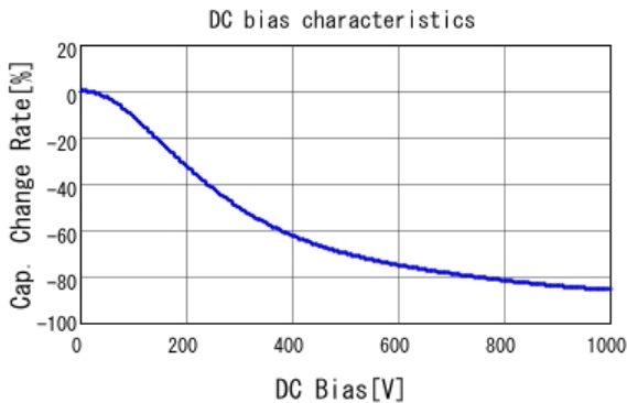
■ GRM55DR73A104KW01 C-DC bias capchange, 25.0degC, AC1V
