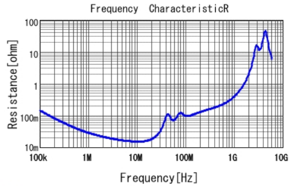
■ GRM55DR73A104KW01 R DC0V, 25degC
