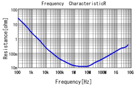
■ GRMMDXR60J105ME05 R DC0V, 25degC
