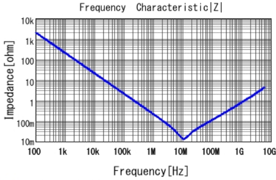
■ GRMMDXR60J105ME05 |Z| DC0V, 25degC
