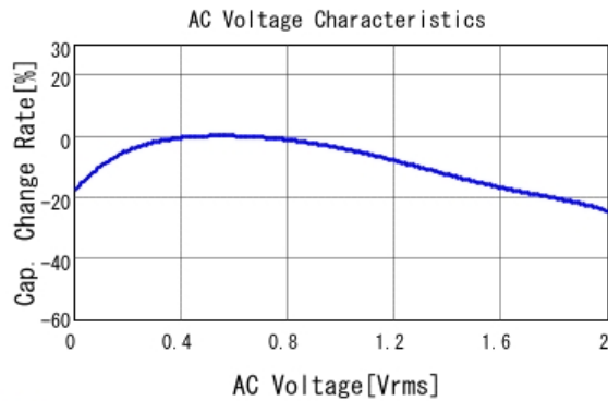
■ GRMMDXR60J105ME05 C-AC Voltage capchange, DC0V, 25.0d
