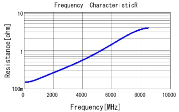
■ GRT0335C1H330JA02 R DCOV, 25degC
