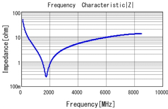
■ GRT0335C1H330JA02 |Z| DCOV, 25degC
