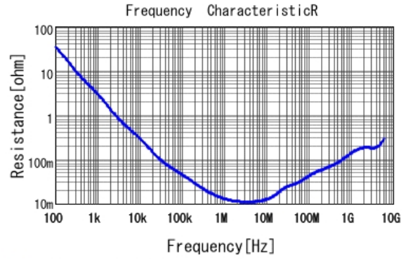
■ GRT033R60J105ME13 R DC0V, 25degC
