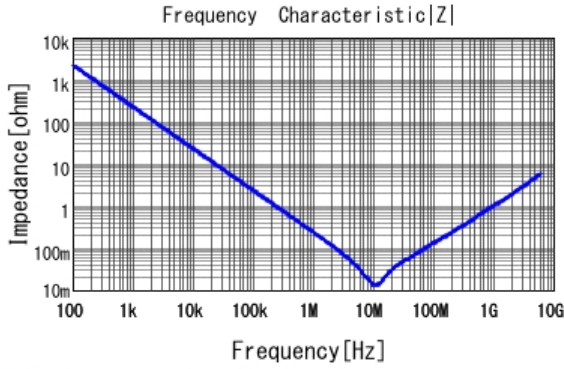
■ GRT033R60J105ME13 |Z| DC0V, 25degC
