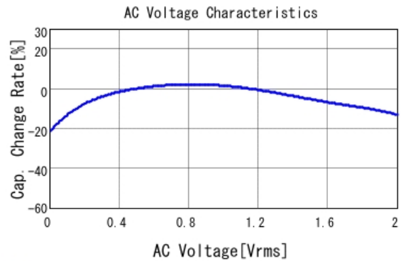
■ GRT033R60J105ME13 C-AC Voltage capchange, DC0V, 25.0d
