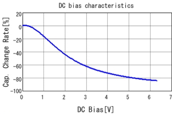
■ GRT033R60J105ME13 C-DC bias capchange, 25.0degC, AC0.
