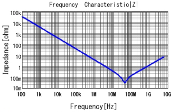
■ GRT033R60J473KE01 |Z| DCOV, 25degC
