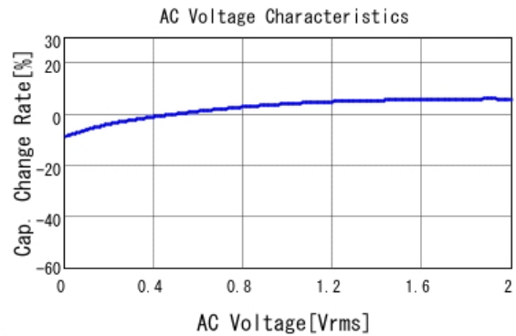
■ GRT033R60J473KE01 C-AC Voltage capchange, DCOV, 25.0d
