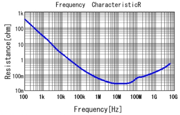
■ GRT033R60J473KE01 R DCOV, 25degC
