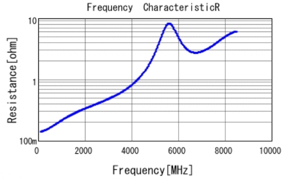
■ GRT1555C1H100JA02 R DCOV, 25degC
