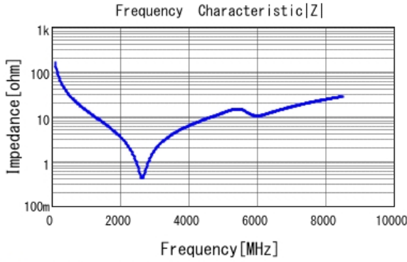
■ GRT1555C1H100JA02 |Z| DCOV, 25degC
