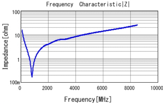
■ GRT1555C1H101JA02 |Z| DCOV, 25degC
