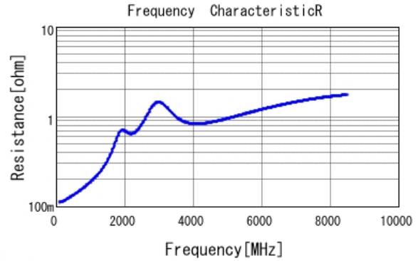
■ GRT1555C1H101JA02 R DCOV, 25degC
