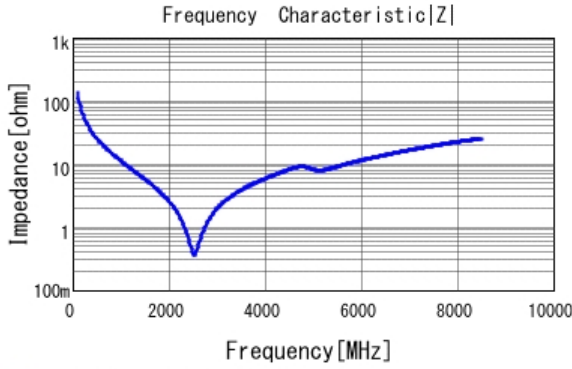
■ GRT1555C1H120JA02 |Z| DC0V, 25degC
