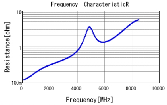
■ GRT1555C1H120JA02 R DC0V, 25degC
