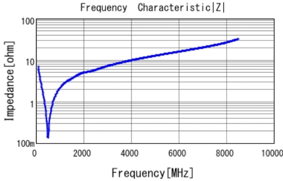
■ GRT1555C1H221JA02 |Z| DCOV, 25degC
