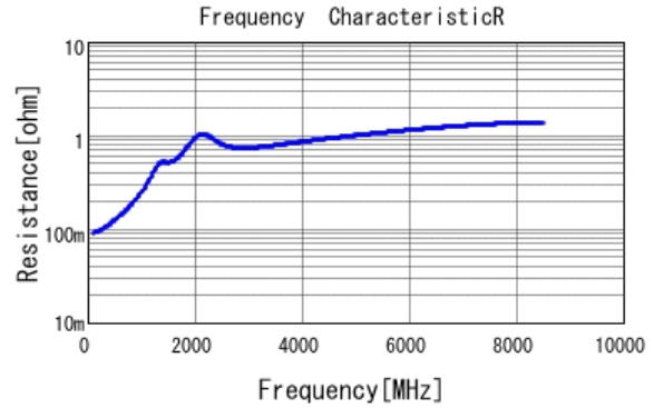
■ GRT1555C1H221JA02 R DCOV, 25degC
