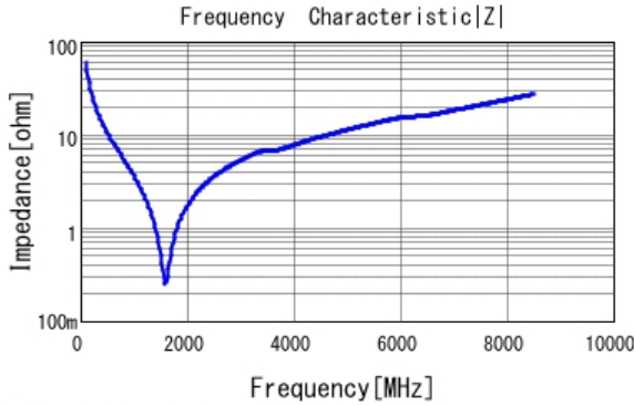
■ GRT1555C1H270JA02 |Z| DCOV, 25degC
