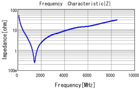
■ GRT1555C1H330JA02 |Z| DCOV, 25degC
