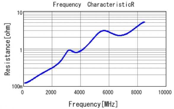
■ GRT1555C1H330JA02 R DCOV, 25degC
