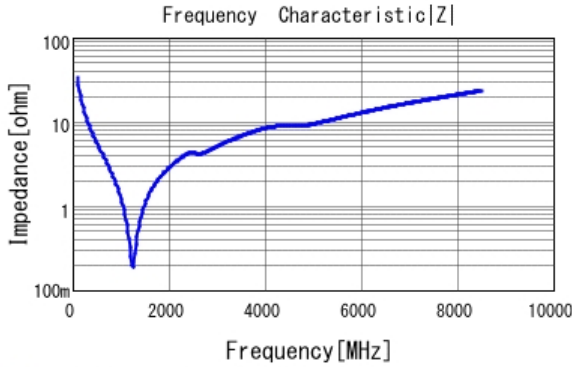
■ GRT1555C1H470JA02 |Z| DCOV, 25degC
