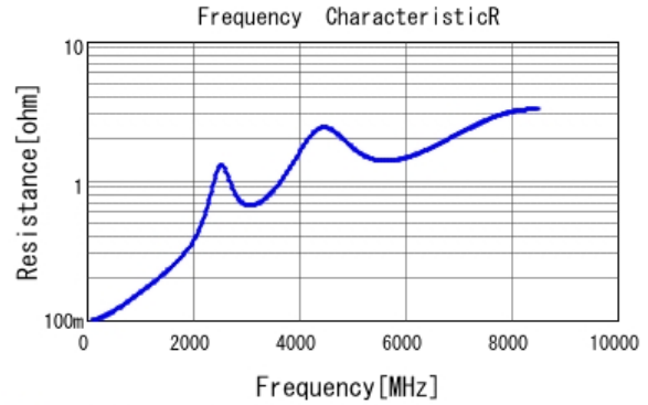
■ GRT1555C1H470JA02 R DCOV, 25degC
