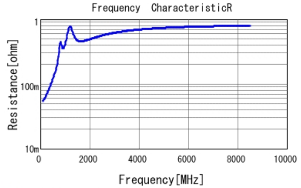
■ GRT1555C1H471JA02 R DC0V, 25degC
