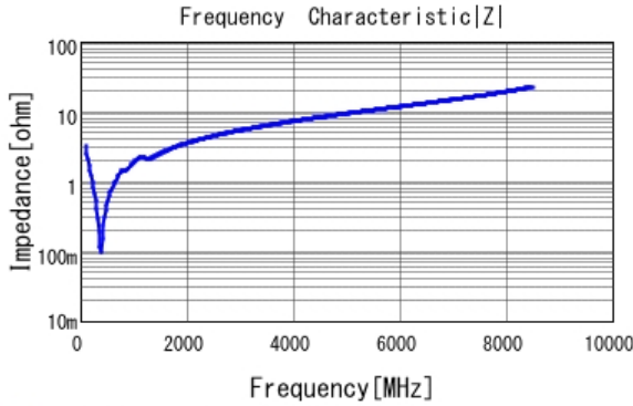
■ GRT1555C1H471JA02 |Z| DC0V, 25degC
