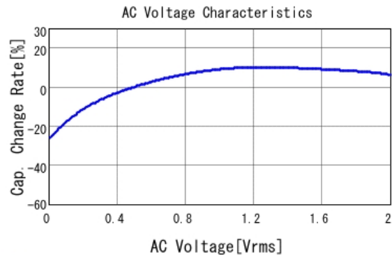
■ GRT155R60J105KE01 C-AC Voltage capchange, DC0V, 25.0d
