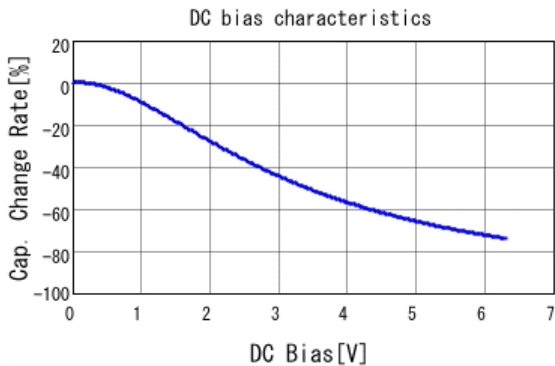
■ GRT155R60J105KE01 C-DC bias capchange, 25.0degC, AC0.
