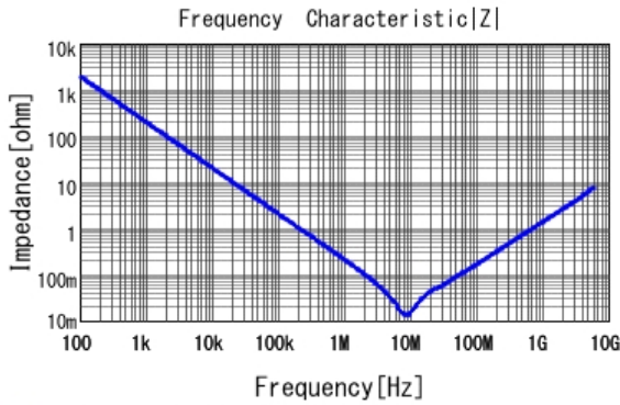
■ GRT155R60J105KE01 |Z| DC0V, 25degC
