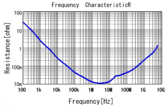
■ GRT155R60J105KE01 R DC0V, 25degC
