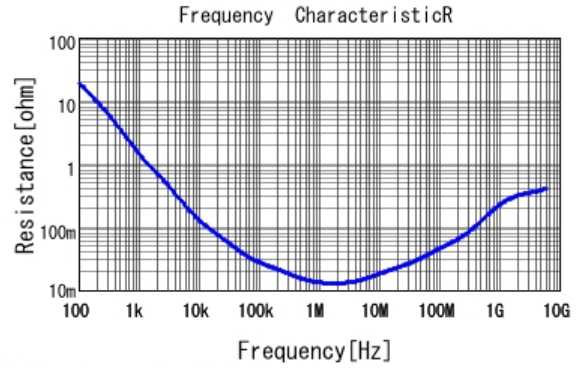
■ GRT155R60J225KE01 R DC0V, 25degC
