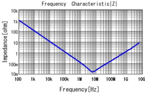
■ GRT155R60J225KE01 |Z| DC0V, 25degC
