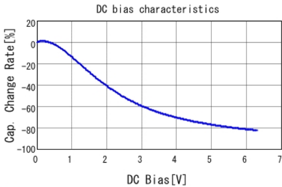
■ GRT155R60J225KE01 C-DC bias capchange, 25.0degC, AC0.
