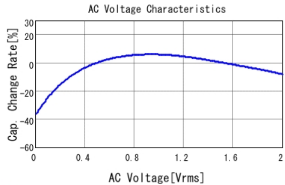
■ GRT155R60J225KE01 C-AC Voltage capchange, DC0V, 25.0d
