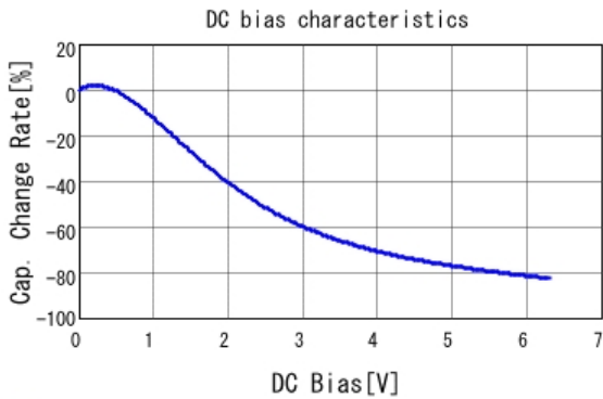
■ GRT155R60J475ME13 C-DC bias capchange, 25.0degC, AC0.
