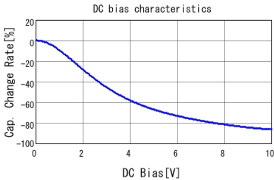
■ GRT155R61A105KE01 C-DC bias capchange, 25.0degC, AC1V
