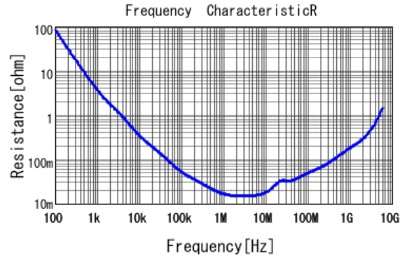
■ GRT155R61A105KE01 R DC0V, 25degC
