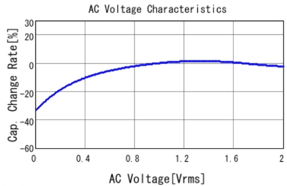
■ GRT155R61A105KE01 C-AC Voltage capchange, DC0V, 25.0d
